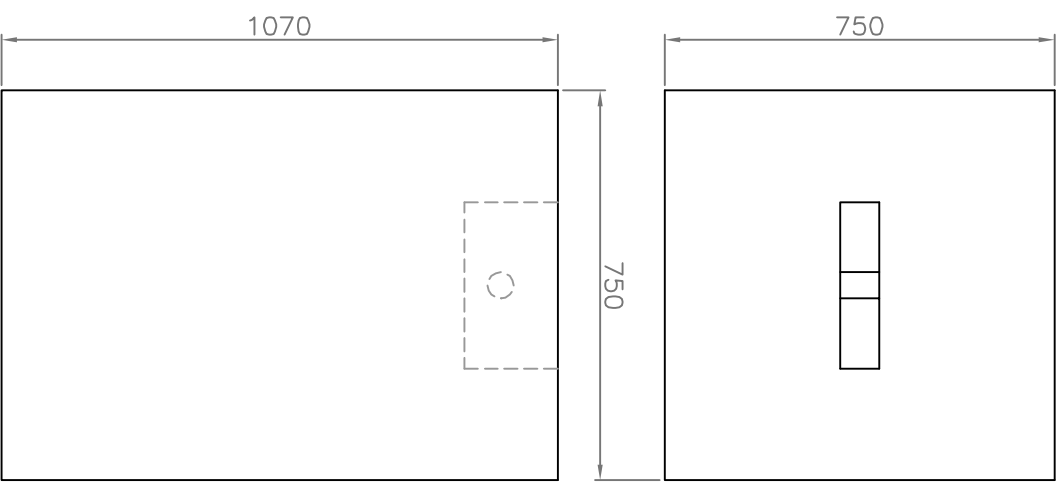
4.4 TONNE TEST WEIGHT 10 OFF
